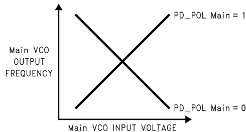
Figure 39. Main VCO Characteristics
